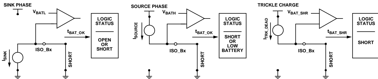
Figure 31. Trickle Charge
